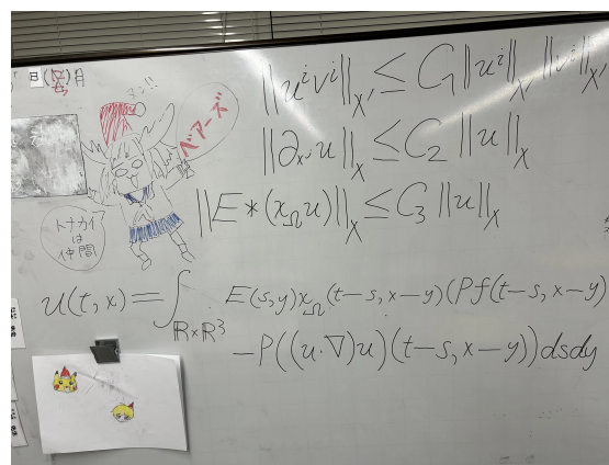
Completion of normed spaces, the graph of E = E(Y, X) , convolutions, and key inequalities.
